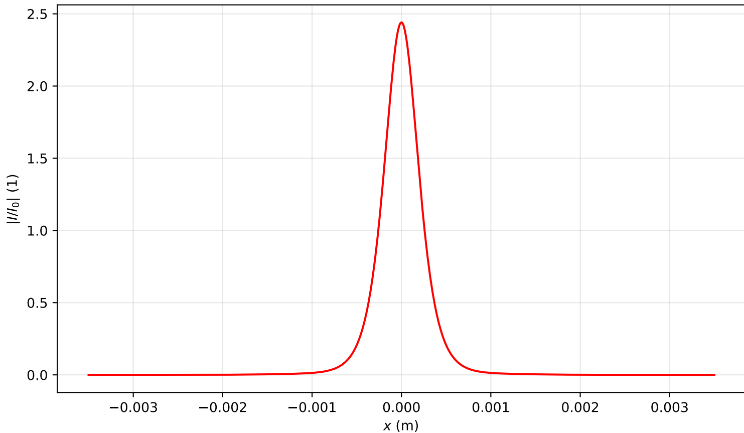
Intensity profile I(x, y = 0, z = 2.627)/I_0 , P_{in}=1.0P_{cr} , artificial time
